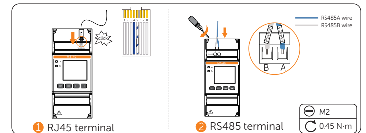
Figure 6-3 Connecting communication cables
