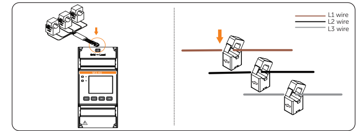
Figure 6-2 Connecting CT cables
