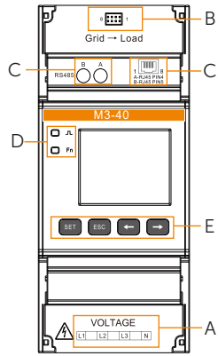
Figure 1-1 M3-40 appearance
